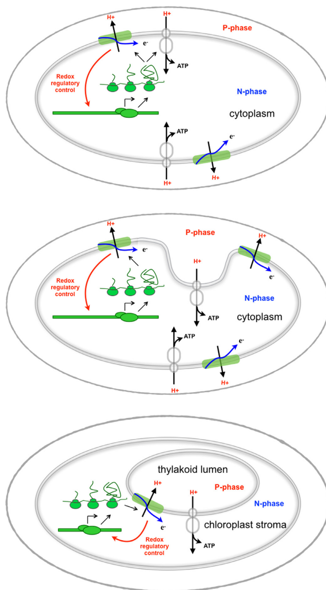
Fig. 3. The direction of electron transport-driven proton translocation in relation to the genetic systems of (i) mitochondria and bacteria (top); (ii) photosynthetic bacteria, including cyanobacteria (middle); (iii) chloroplasts (bottom) where the thylakoid membrane has been inverted and sealed off from the cell membrane from which it evolved, thus enclosing the thylakoid lumen (the P-phase) and separating it from the chloroplast stroma (the N-phase), which is homologous with the bacterial cytoplasm. A schematic bioenergetic-genetic system of DNA, RNA, ribosomes and polypeptides is depicted in green, as in Fig. 1, and is located in the N-phase in all cases. (For interpretation of the references to colour in this figure legend, the reader is referred to the web version of this article.)
