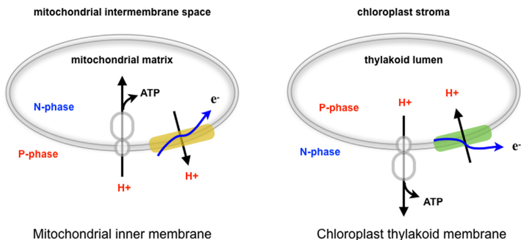
Fig. 2. The direction of electron transport-drive proton translocation in isolated mitochondrial inner membranes (left) and chloroplast thylakoids (right).
